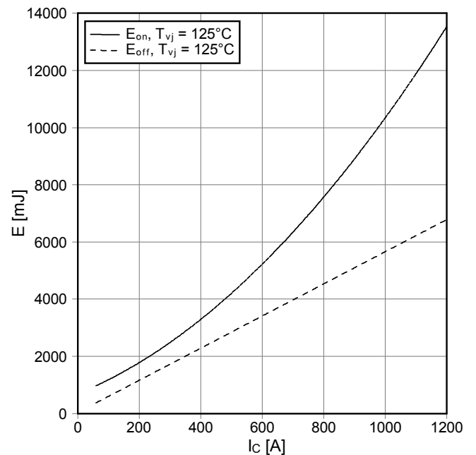
Schaltverluste IGBT-Wechselr. (typisch) switching losses IGBT-inverter (typical) E_{on} = f(I_c), E_{off} = f(I_c) V_{GE} = \pm 15\text{ V}, R_{Gon} = 1.3\ \Omega, R_{Goff} = 8.2\ \Omega, V_{CE} = 3600\text{ V}
